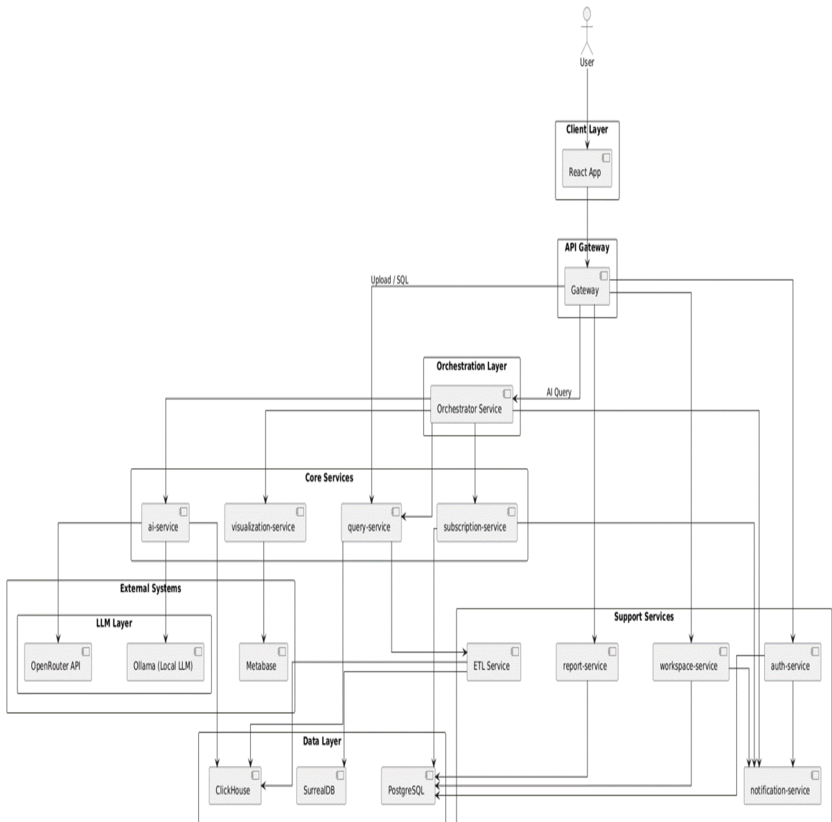
Figure 41 : System Architecture
