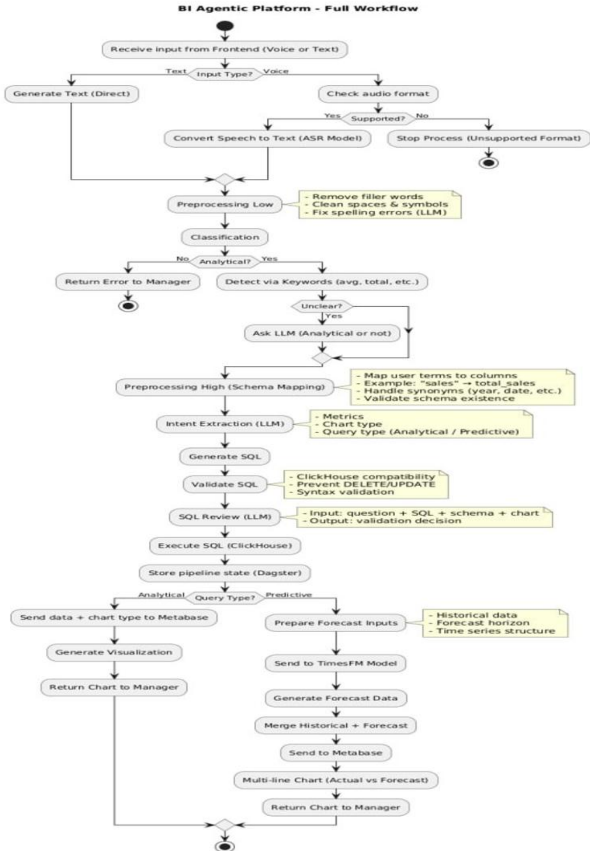
Figure 48 : AI Processing Pipeline
